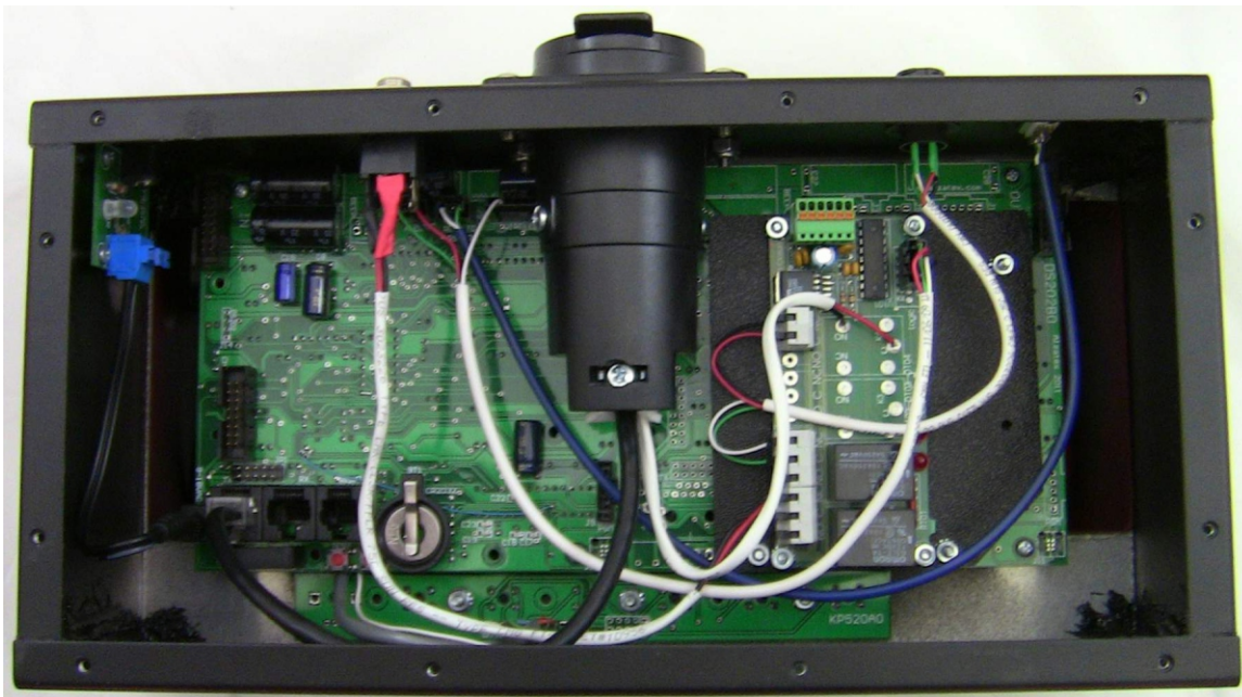
View of the inside of the DSP254B6-BSC controller showing the optional relay board.
